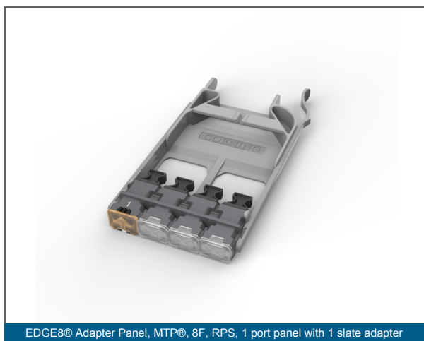
EDGE8® Adapter Panel, MTP®, 8F, RPS, 1 port panel with 1 slate adapter
